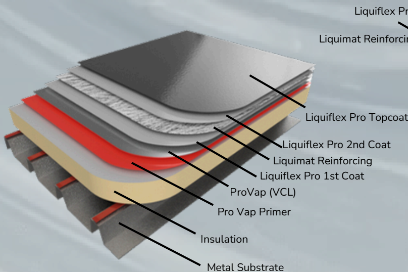
20 YEAR SYSTEM WITH A WARM ROOF BUILD UP
