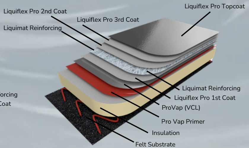
25 YEAR SYSTEM WITH A WARM ROOF BUILD UP
