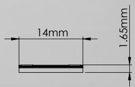
Affinity Magnetic Track
