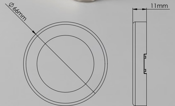
Affinity Magnetic Track Cover
