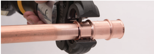
1. Insert the tube in the fitting
