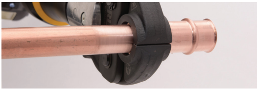
3. Activate the battery-powered tool
