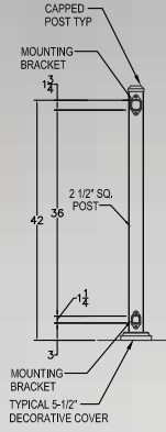
2-LINE RAILING DETAIL
