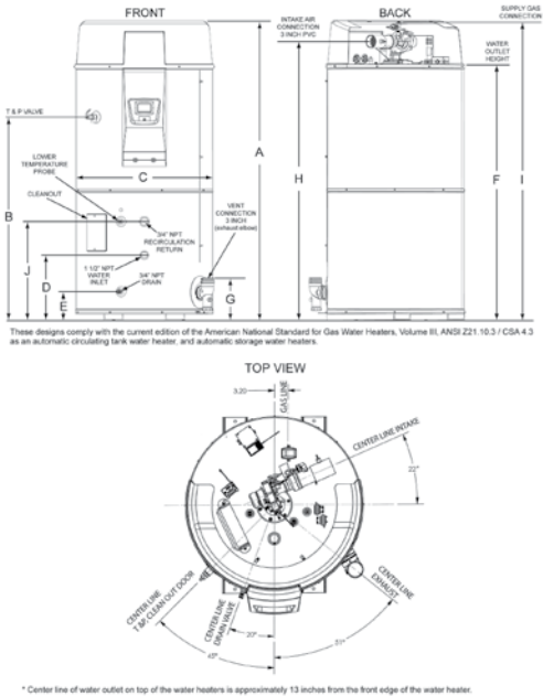
Figure 5. Rough-In Dimensions
