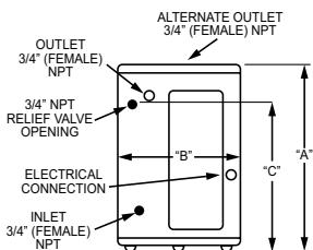
FRONT VIEW DEL 6/10/15/20
