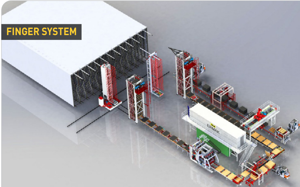
"L" SYSTEM - LEG PALLET
