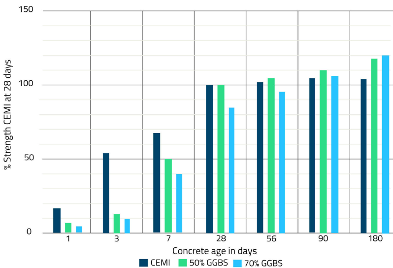
Graph 1 - Comparative strengths of CEM I 50% and 70% GGBS Concretes
