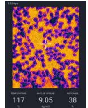
Above: Optional VISIR-ROS uses a thermal imaging camera to differentiate between cold chippings and hot rolled asphalt.
