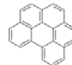
Benzo(g,h,i)perylene
