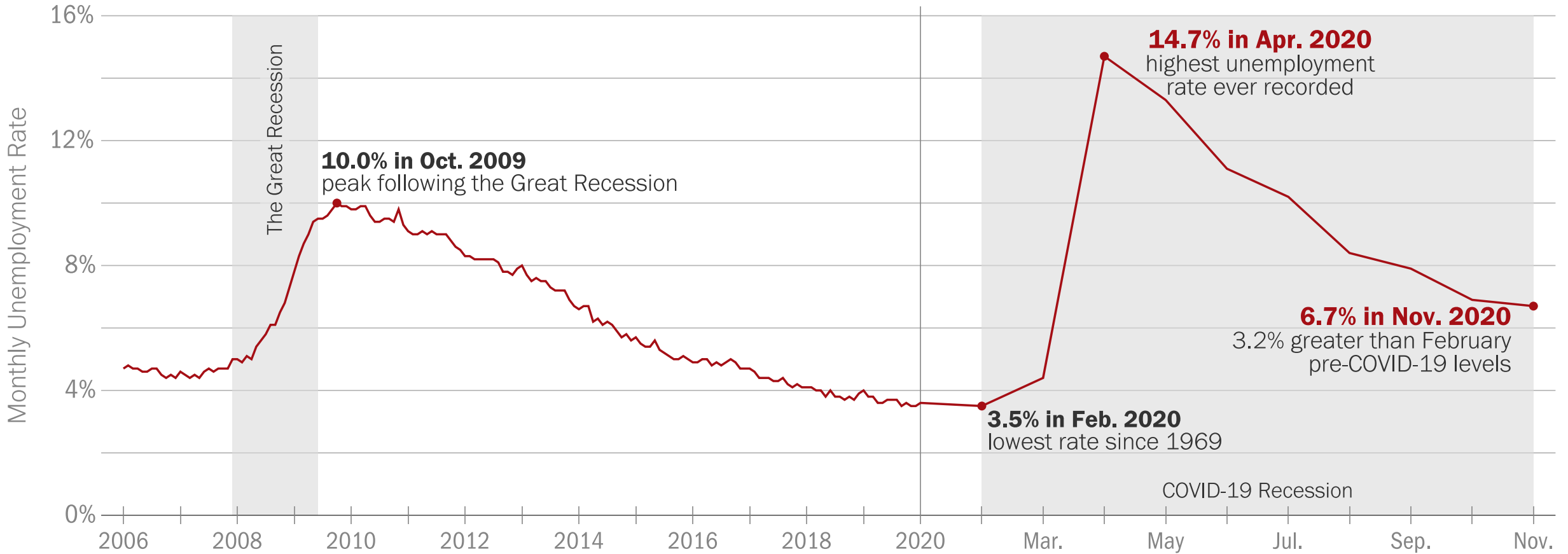
U.S. unemployment rate, 2006- Nov. 2020
